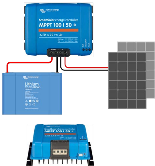
Figure 1: Power connections
